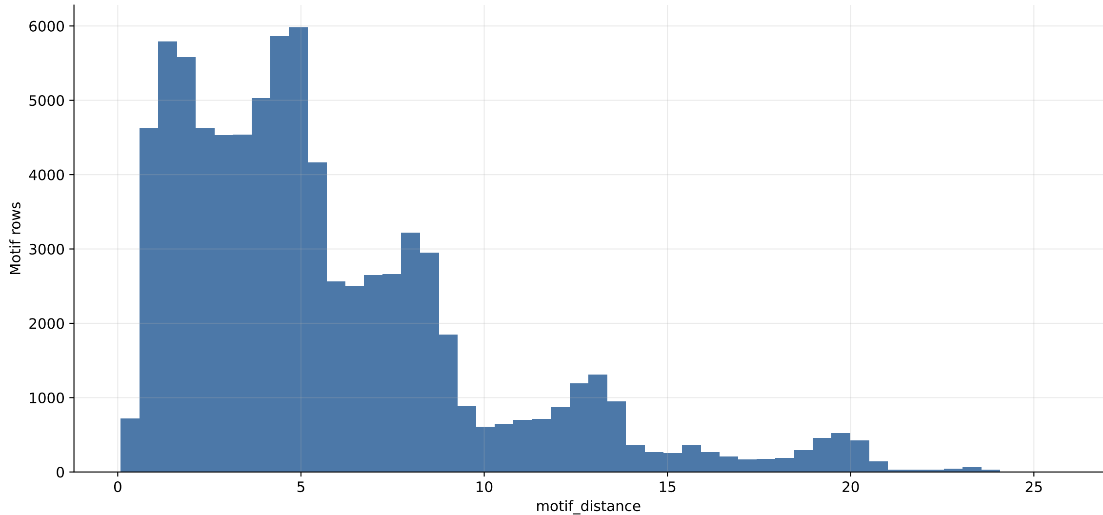
Matrix Profile motif distance distribution, overall
